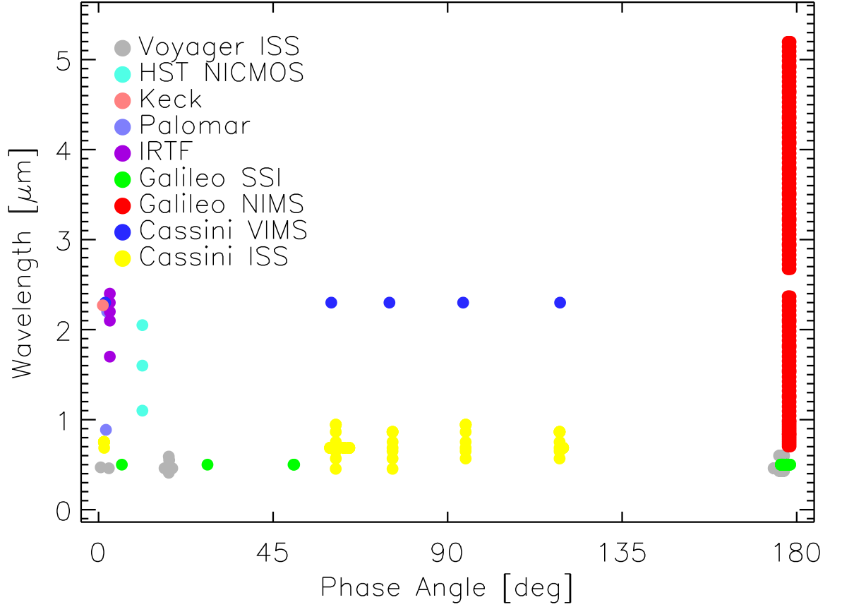
Fig. 3.— ‘Phase space’ of observations of the Jovian ring. Cassini’s ISS (yellow) and VIMS (blue) have filled in significant regions of phase angle that were previously unexplored. The densest region of points remains a spectral cube of the ring obtained by the Galileo NIMS instrument (red); all Earth-based observations are at the left, at \alpha < 12^\circ .
