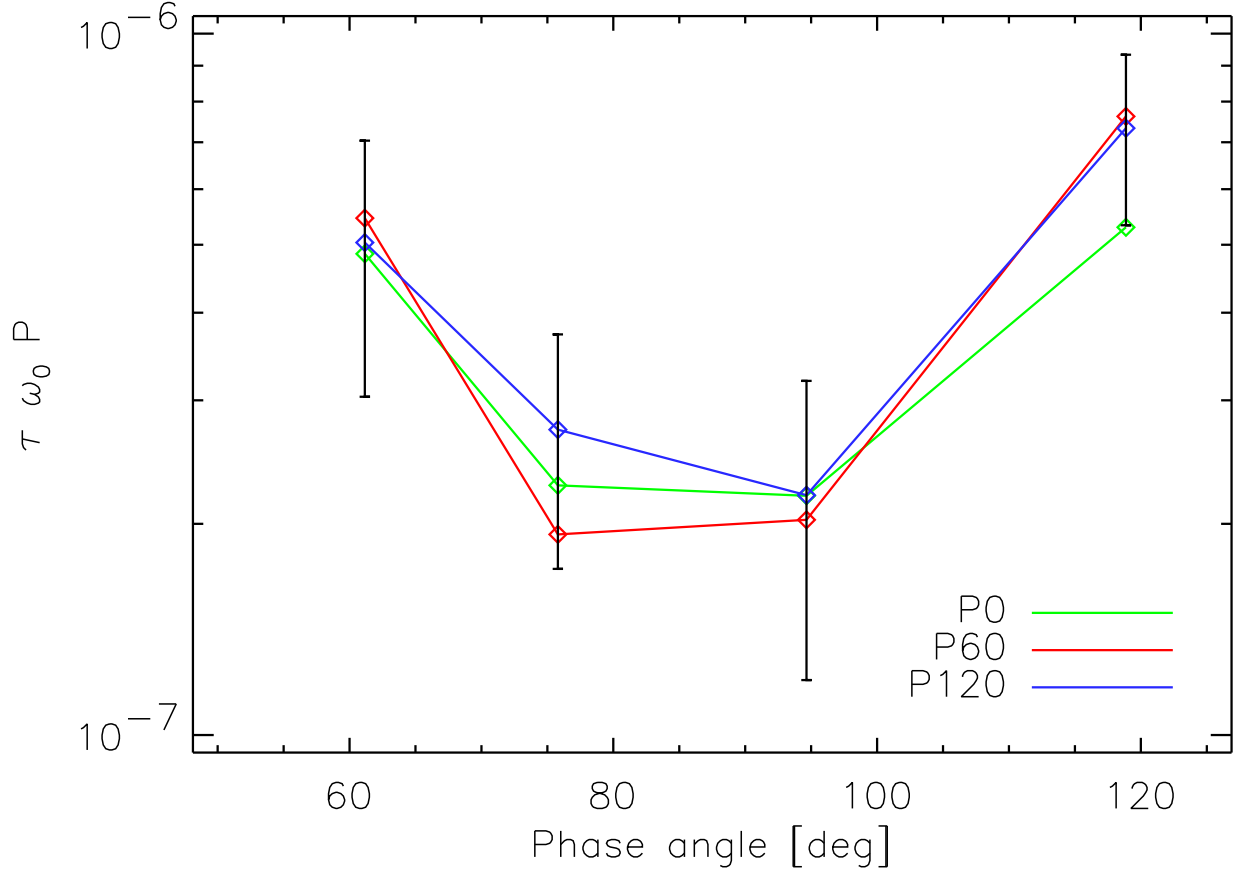
Fig. 10.— ISS polarization observations. The ring was observed in a clear filter at three polarization angles, denoted by P0, P60, and P120. Error bars have been taken from comparable non-polarized observations. Because only one frame was taken for each data point, the uncertainty is large and dominates any observable difference at the three polarization angles.
