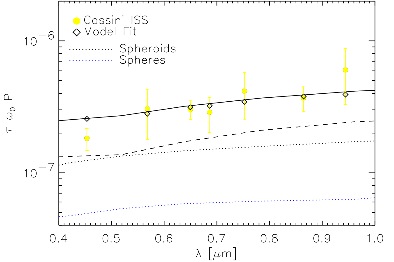
Fig. 6.— Composite ring spectrum, for \alpha \sim 75^\circ . The ring is red, with I/F increasing almost linearly with wavelength. Symbols are the same as in Fig. 4. In our best fit model, the ring’s color is due predominantly to that from the large bodies, suggesting that they must be very red. The dotted blue line (which is a separate calculation for spheres alone) indicates that the spectrum from spherical particles is very similar to that of non-spherical ones.
