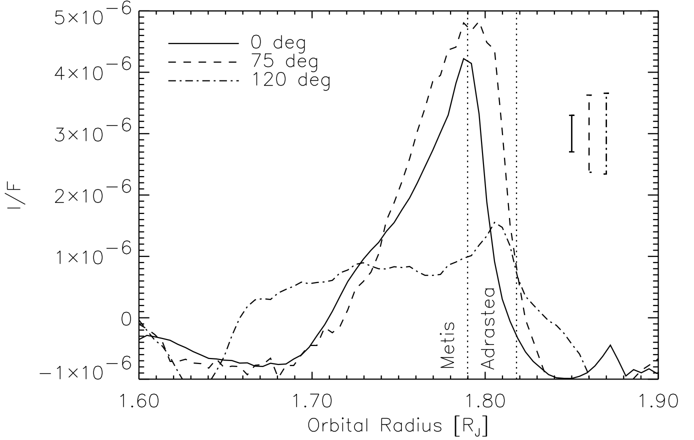
Fig. 7.— Radial profiles of the ring. At \alpha = 120^\circ , the profile is broad but of low magnitude, consistent with the small particles predominantly seen at forward-scatter. In contrast, the backscatter profiles at \alpha = 0^\circ and \alpha = 75^\circ show the tighter concentration of large bodies toward the ring’s outer edge. Error bars for each curve are indicated at the right; errors in orbital radius are approx \pm 0.02 R_J .
