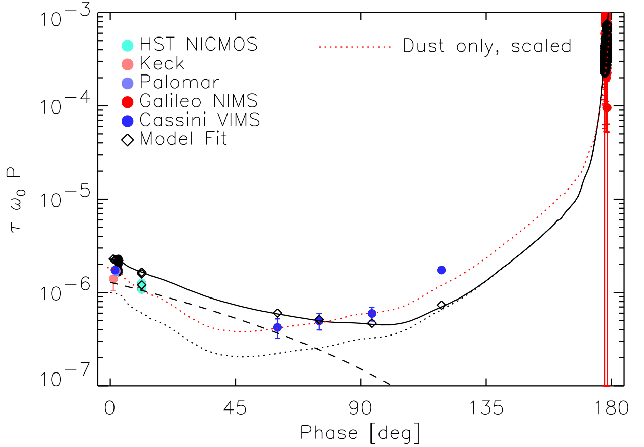
Fig. 16.— Infrared phase curve for data points with \lambda = 1 - 2.5 \mu\text{m} . Symbols are the same as in Fig. 4. The best-fit model provides only a fair fit to the VIMS data. However, the phase curve of the dust alone (red curve) matches quite well, suggesting that the large bodies could be quite dark at the \lambda = 2.3 \mu\text{m} wavelength of the VIMS observations.
