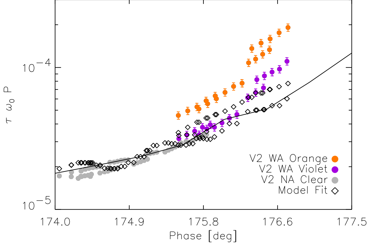
Fig. 17.— Phase curve of Voyager observations. Our solution fits the slope of each segment; variations in the offset between different images are due to in part to calibration uncertainties near image corners in the Voyager observations, and in part to actual differences in the near & far arms of Jupiter seen by Voyager.
