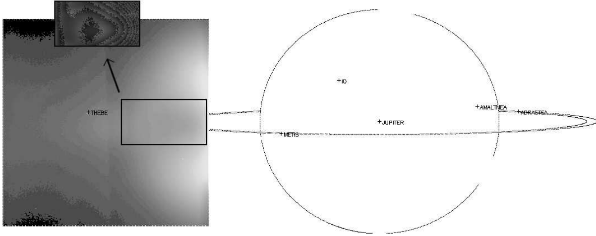
Fig. 1.— Geometry for the inbound movie sequence, for phase angle \alpha \sim 1^\circ and ring opening angle B \sim 3.4^\circ , December 11, 2000. This is a clear-filter image, 1 sec exposure, from 270 R_J . Because the full disk of Jupiter is lit and the projected distance to the ring is \sim 0.5 R_J , the ring is visible above the stray light only after extensive processing. The ‘wood grain’ patterns in the inset image are artifacts of stray light removal over the lookup table used in compressing the image. Images in later sequences are less affected by stray light, because of Jupiter’s increasing phase angle and the spacecraft’s decreasing range (and thus increasing angular separation between the planet and its ring).
