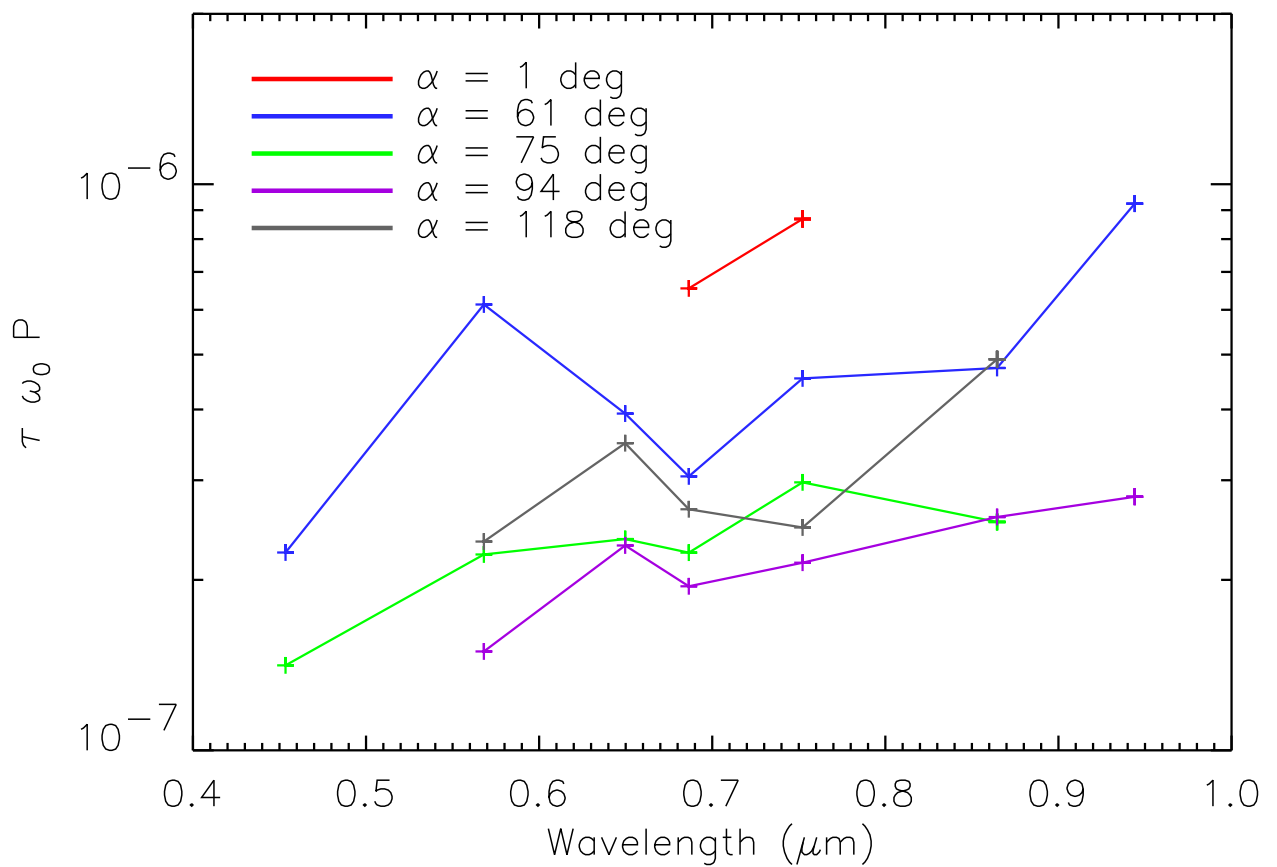
Fig. 5.— Cassini ISS observations of the ring’s spectrum. The ring’s red color is roughly uniform across a wide range of phase angles. A composite mean spectrum from these data points is shown in Fig. 6.
