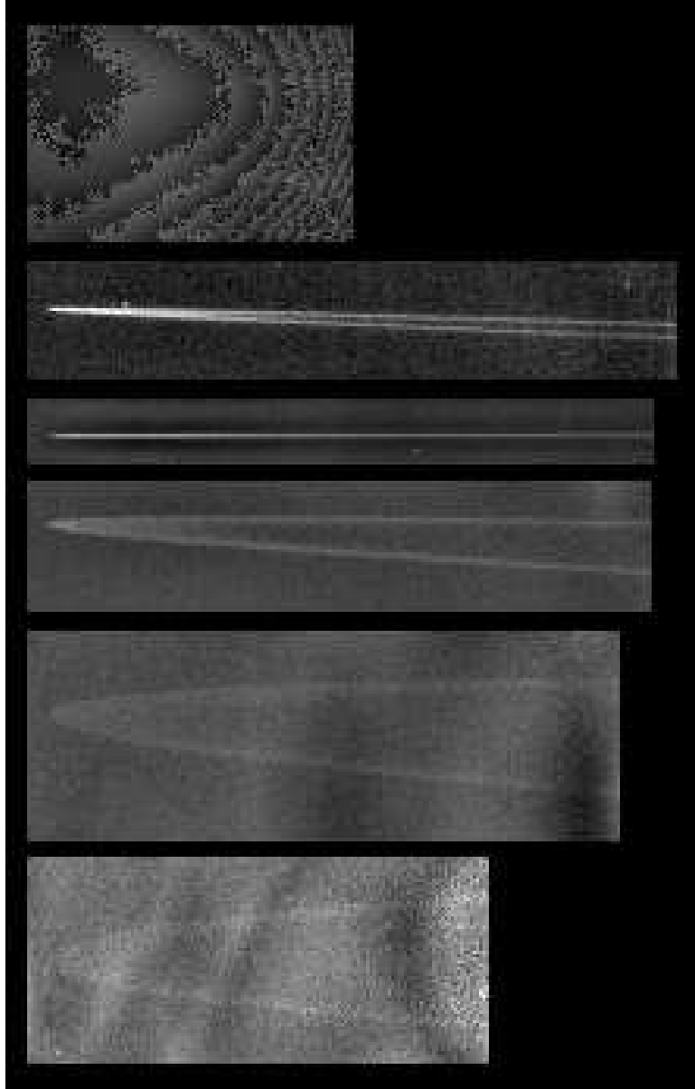
Fig. 2.— The Jovian ring as seen by Cassini from December, 2000 – January, 2001. The phase angles are approximately 1^\circ , 60^\circ , 64^\circ , 75^\circ , 94^\circ , and 120^\circ , while the ranges are approximately 270 R_J , 137 R_J , 137 R_J , 141 R_J , 162 R_J , and 247 R_J . All images are taken through clear filters, with exposure lengths of several seconds. Stray light increases as Cassini leaves the system and the ring once again appears closer to Jupiter. The spatial resolution across these images varies from 120 \text{ km pix}^{-1} at the ends, to 59 \text{ km pix}^{-1} near the 136 R_J closest approach. Images have been rescaled in brightness. Figure from Porco et al. (2003).
