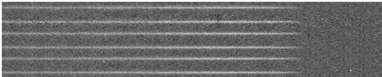
Fig. 11.— The ring’s right ansa, as seen in five images taken at an elevation B = -0.03^\circ . As shown in Fig. 13, these images show only the ring’s near arm. The five clear-filter images have exposures of 1.5–18 sec, and span a total of \sim 5 minutes. The top image has been resampled from the lower SUM2 resolution; the checkerboard patterns in the bottom images is an artifact of our dark-current subtraction.
