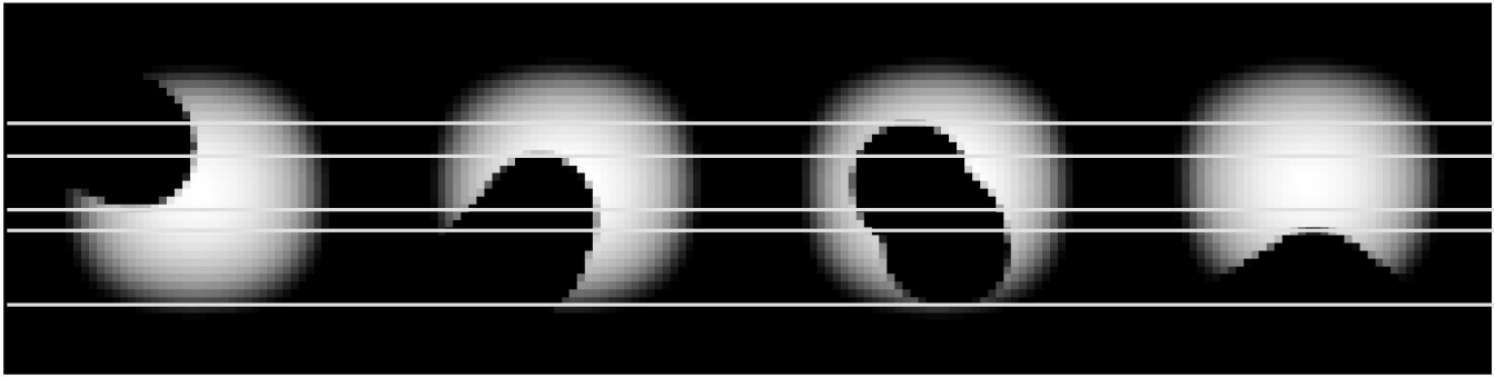
FIG. 4.—Transit paths from the four events, showing Pluto's projected disk with the coverage by Charon's disk and/or shadow. The middle two events are shown at the end of observations; if they had progressed further, Charon's obscuration would have continued to the right across Pluto's disk. In theory we can resolve latitudinal structure within the six delineated bands.
