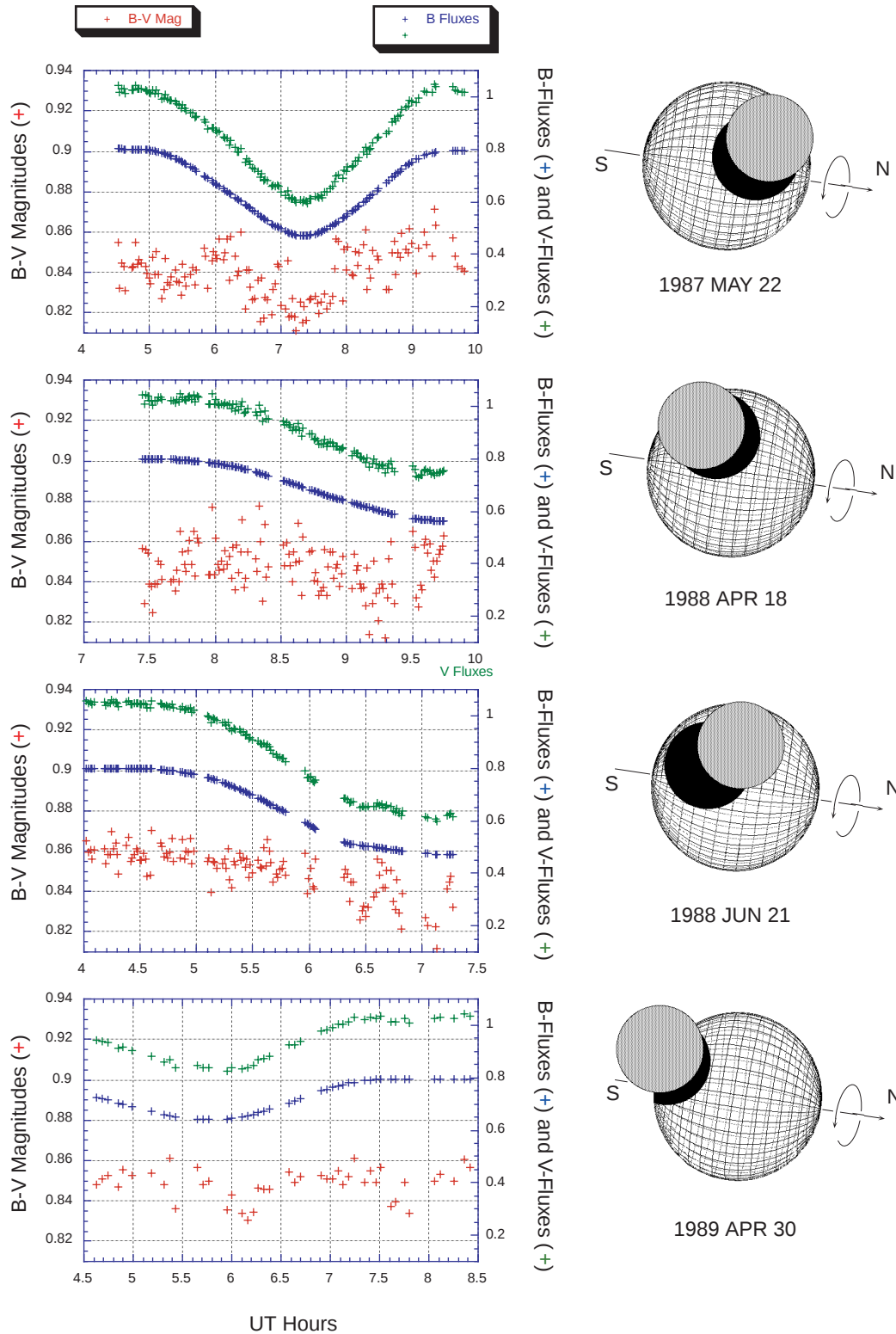
FIG. 3.— B-V magnitude light curves, with B -flux and V -flux light curves. The B -flux light curve is generated by passing an existing B -map through the geometry of these four events, and the V -flux light curve is offset from the B -flux by an amount based on the B-V magnitude differences. Notice that the two 1988 events were only observed through first and second contact (i.e., the ends of the transits were not observed) and that the 1989 event was picked up after first contact.
