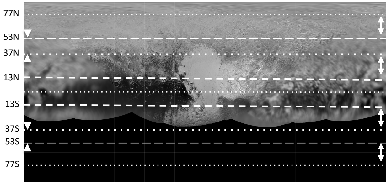
Fig. 6. Climate zones on Pluto and their geographic expression. The division between the arctic and diurnal climate zones oscillates between \pm 13^\circ and \pm 37^\circ , and the division between the tropic and polar climate zones oscillates between \pm 53^\circ and \pm 77^\circ . The base of each triangle on the left indicates the current location of each zone boundary while pointing in the direction of the boundary's current migration. The area between \pm 13^\circ is a permanent diurnal zone, which experiences sunrise and sunset every Pluto day. The area between \pm 53^\circ is the zone of permanent tropics, where the Sun always reaches the zenith at least once per orbit. Poleward of \pm 37^\circ is the permanent arctic zone, which always experiences arctic seasons, up to century-long summers and winters during each orbit. Poleward of \pm 77^\circ is the permanent polar zone, where the Sun never reaches zenith over any orbital period. Adapted from Binzel et al. (2017).
