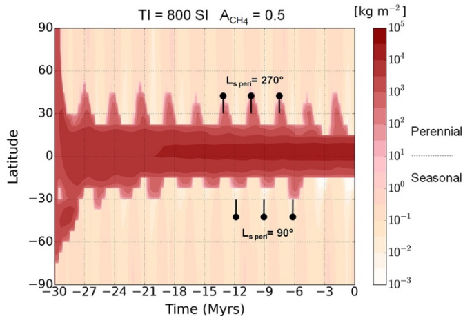
Fig 13. Example run for an initially global CH_4 with A_{CH_4} = 0.5 , showing the zonal annual mean of CH_4 outside of Sputnik Planitia.
