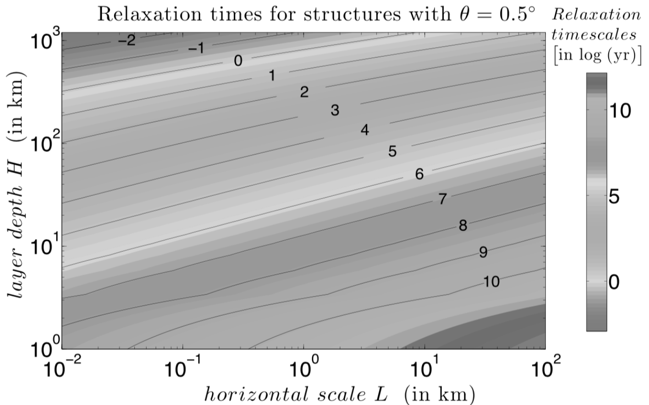
Fig. 8 From Umurhan et al. 2017 (see Umurhan et al. 2017 for color version). Relaxation timescale for glacial flow over shallow slopes. The timescale for filling in depressions by atmospheric transport at current Pluto temperatures is about 10^7 years. Thus, atmospheric transport is shorter (more efficient) than glacial flows for shallow deposits or deposits separated by large distances. Moreover, atmospheric transport operates even when the source and sink areas are discontinuous, as is more likely for shallow deposits and large separations.
