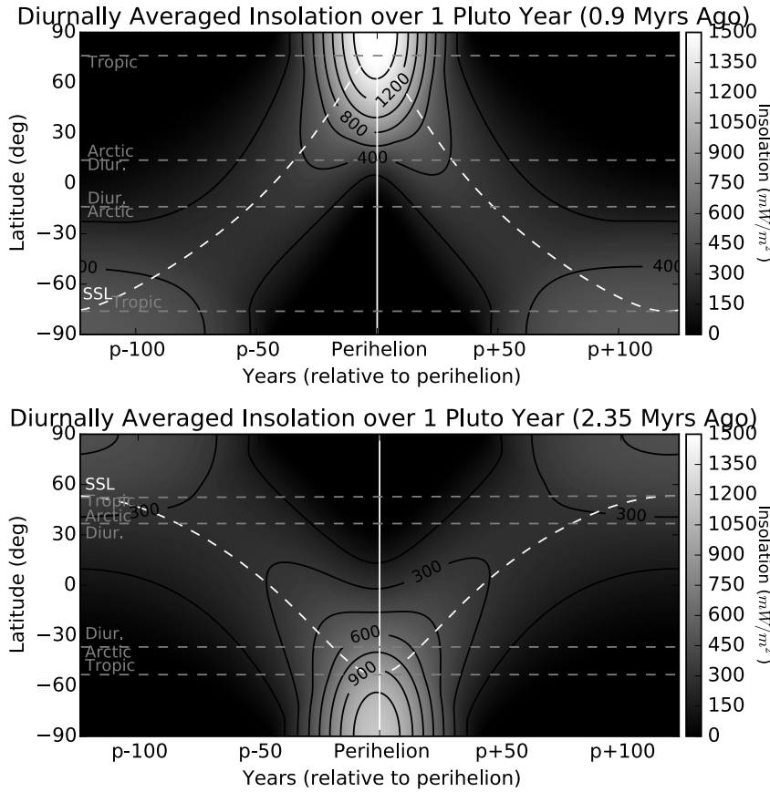
Fig. 7. Diurnally averaged insolation over one Pluto year for two different epochs, with the subsolar latitude (SSL), tropics, and the diurnal/arctic division plotted as in Fig 5-XX, Middle. Top: Northern summer solstice at perihelion ( L_{s,peri} = 90^\circ ) at a time of high obliquity. Bottom: Southern summer solstice at perihelion ( L_{s,peri} = 270^\circ ) at a time of low obliquity.
