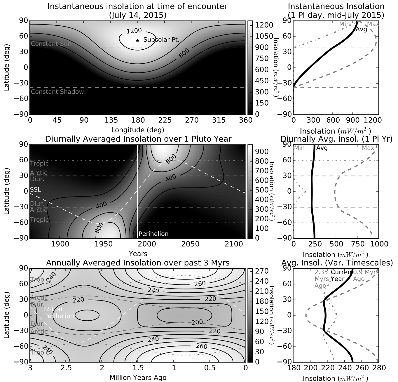
Fig. 5. Incident solar flux (insolation) on Pluto at various timescales. Contour labels are in \text{mW m}^{-2} . (Top) Insolation over one Pluto rotation at the time of New Horizons flyby, with longitudes relative to midnight. (Middle) Diurnally averaged insolation over one Pluto year, with the subsolar latitude (SSL) shown as a white dashed line. Also plotted in gray are critical latitudes: the tropics at \pm 61^\circ , between which the sun is overhead at some time in the year; and the arctic/diurnal division at \pm 29^\circ , between which sun rises and sets every day of the year, and beyond which the latitude experiences arctic night sometime during the year. (Lower) Annually averaged insolation.
