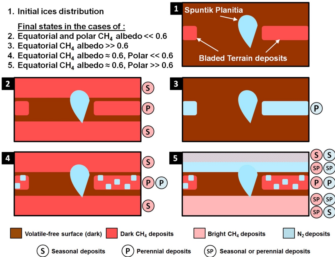
Fig 14. Summary of the simulation results for runs with that were initialized with N 2 in Sputnik Planitia, and an infinite reservoir of CH 4 at the latitudes of the bladed terrain (Bertrand et al. 2019; their Section 4).
