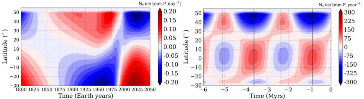
Fig. 11. Left: Evolution of the diurnal mean condensation-sublimation rate within Sputnik Planitia (mm per Pluto day; red is condensation), in current orbital conditions, from 1800 to 2050 assuming that the glacier remains flat. Right: Evolution of the annual mean condensation-sublimation rate of N_2 ice with time (mm per Pluto year; red is condensation), assuming that the glacier remains flat (same as Fig. 8. The vertical solid and dashed lines correspond to the periods of high ( 104^\circ ) and low ( 127^\circ ) obliquity, respectively
