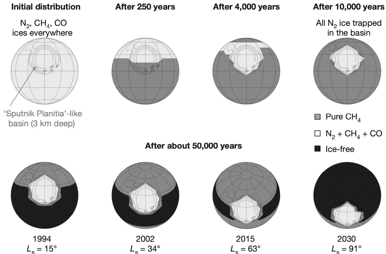
Fig. 10. Surface maps from the reference simulation of BF16 with thermal inertia = 800 tui. Top: The evolution beginning with all ices uniformly distributed. Bottom: Four views of the seasonal evolution of the CH 4 ice (the N 2 ice remains sequestered in Sputnik Planitia). See Bertrand and Forget (2016) for the original figure (in color).
