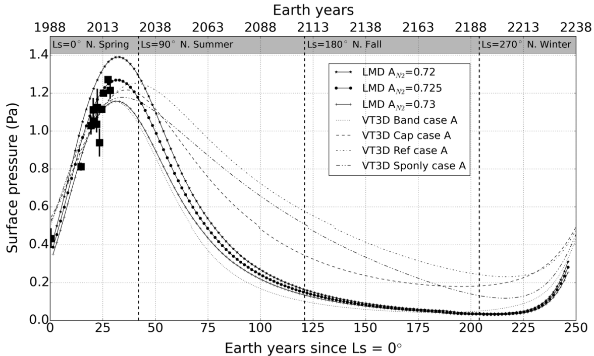
Fig 12. Dashed: four models of pressure over a Pluto season for four assumptions of a static N_2 -ice distribution from Johnson et al. (2020): Sputnik only (Sponly); the N_2 -presence map of Lewis et al. (2020) (Ref); the N_2 -presence map plus a southern N_2 polar cap (Cap); or the presence map plus a southern N_2 mid-latitude band (Band). Solid: Three models of pressure over a Pluto season from Meza et al. (2019).
