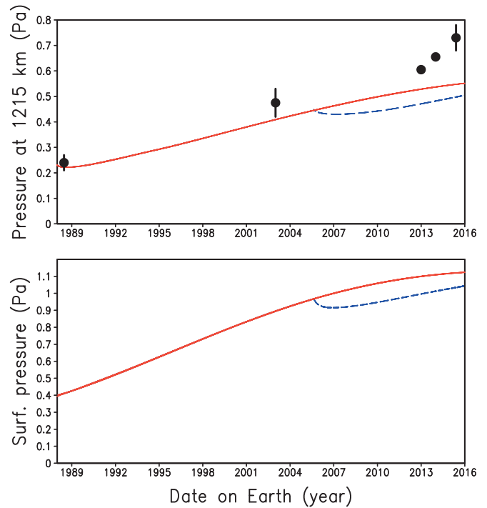
Fig. 2. Evolution of the pressure at r = 1215 km from the planet center (Top) and of the global mean surface pressure (Bottom) in the reference simulation with no south pole N_2 condensation (red solid line) and in the alternative simulation with south pole N_2 condensation (blue dashed line) starting at the end of 2005. The black dots with error bars show the pressure data at r = 1215 km obtained by stellar occultations, as compiled by Sicardy et al. (2016). (For interpretation of the references to colour in this figure legend, the reader is referred to the web version of this article.)
