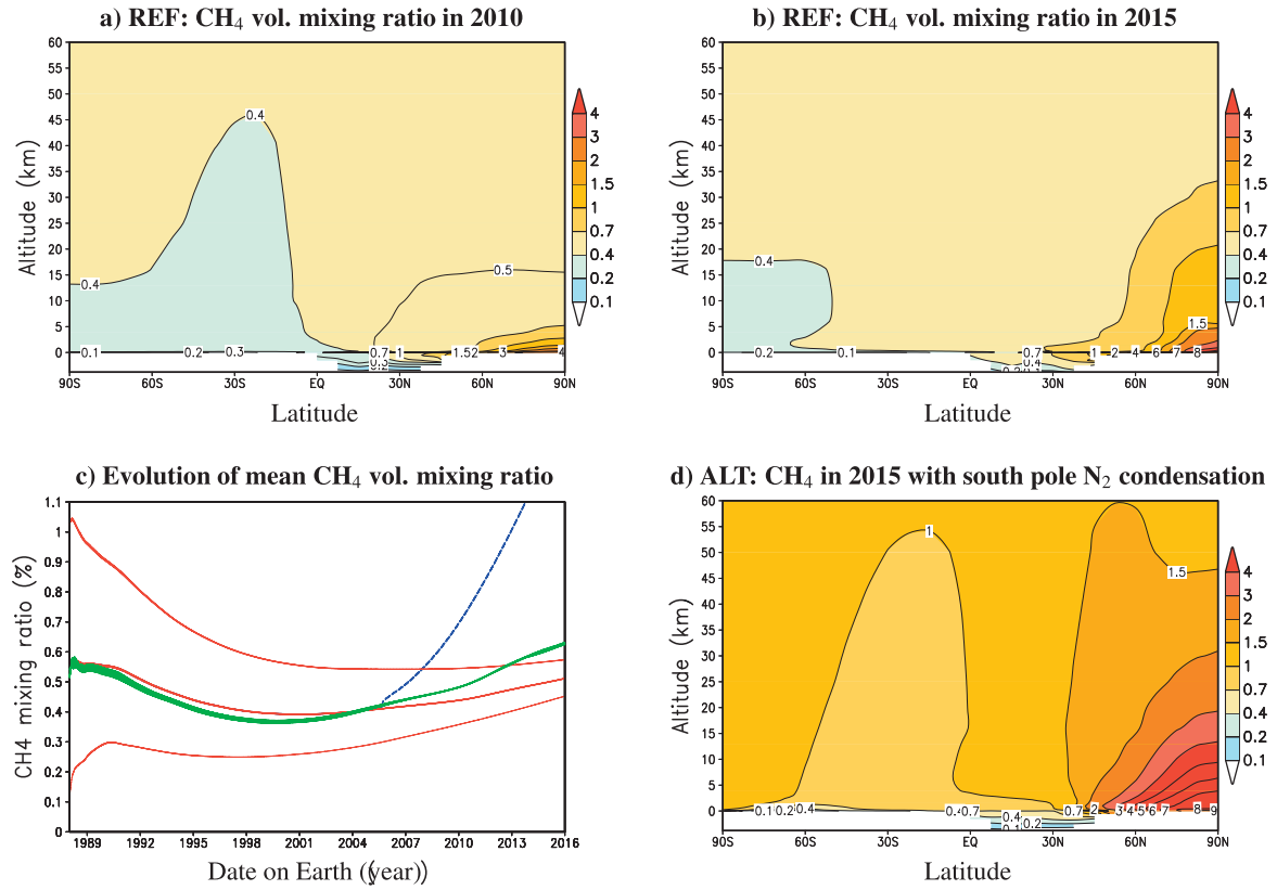
Fig. 12. a) - b): Zonal mean methane volume mixing ratio (%) in the reference simulation (without south pole N 2 condensation and [CH 4 ] initially at 0.5% in 1988) in 2010 and 2015. c): Evolution of the mean volume mixing ratio: globally averaged with different initialization (red), the apparent mixing ratio as seen from the Earth (green, see text) and in the alternative simulation with south pole N 2 condensation started in 2005 (dashed blue). d): Zonal mean methane volume mixing ratio (%) in the alternative simulation (with south pole N 2 condensation) in 2015. (For interpretation of the references to colour in this figure legend, the reader is referred to the web version of this article.)
