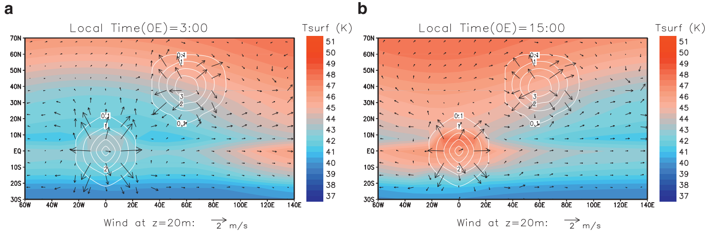
Fig. 4. Maps of surface temperature and winds at 20 m above the surface in July 2015 in the sub-charon hemisphere, where two artificial 4000 m-high mountains has been added to illustrate the formation of downward slope winds on Pluto. The topography is shown by white contours. The local time at longitude 0°E is 3:00 (nighttime) and 15:00 (daytime).
