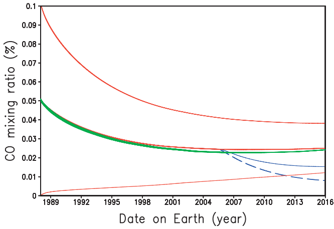
Fig. 15. Evolution of the mean volume mixing ratio of gaseous carbon monoxide. The red curves present the globally averaged values with different initialization. The green curve shows the apparent mixing ratio as seen from the Earth. The blue curves shows the global mean mixing ratio in the alternative simulation with south pole N_2 condensation started in 2005 (see text). (For interpretation of the references to colour in this figure legend, the reader is referred to the web version of this article.)
