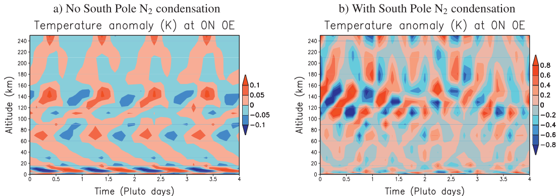
Fig. 9. Temperature anomaly (difference between instantaneous value and diurnal average) at 0°E–0°N in the reference and alternative simulations in July 2015. Thermal tides are clearly visible in the reference simulation, whereas the alternative simulation is characterized by atmospheric barotropic waves (see text).
