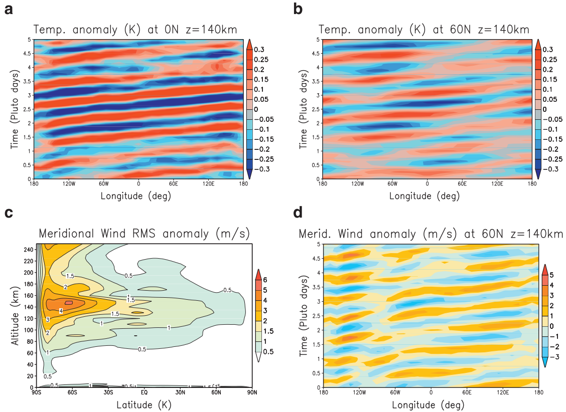
Fig. 11. Characteristics of the barotropic waves present in the simulations with South Pole \text{N}_2 condensation inducing a condensation flow. a) Hövmøller diagram of the temperature anomaly (difference between the local and the zonal-mean temperature) at 0°N. b) Same at 60°N. c) Zonal average of the root-mean-square standard deviation of the local meridional wind from the zonal-averaged meridional wind. d) Hövmøller diagram of the meridional wind anomaly (difference between the local and the zonal-mean wind, in \text{m s}^{-1} ) at 0°N.
