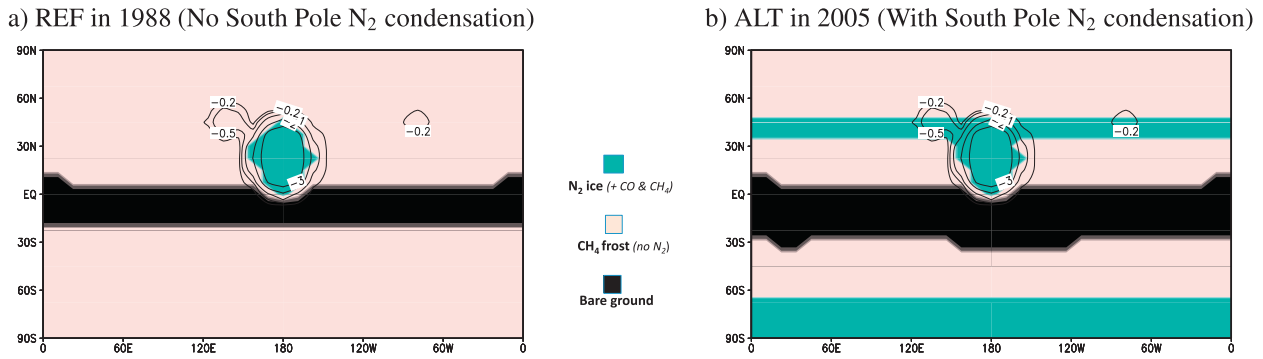
Fig. 1. Maps of surface ice distribution and topography at the beginning of the reference and alternative simulations presented in this paper. The black lines show the assumed topography contours (km). a): Initial state of the reference simulation with no N_2 condensation in the south polar region, in Earth year 1988. This state is the outcome of a 40,000-Earth-years simulation performed with the reduced 2D model. b): Initial state of the alternative simulation with N_2 condensation in the south polar region, in Earth year 2005. This state is derived from the reference simulation state in 2005, with nitrogen added between 35^\circ N and 48^\circ N and subsurface temperature poleward of 65^\circ S decreased by 0.5 K.
