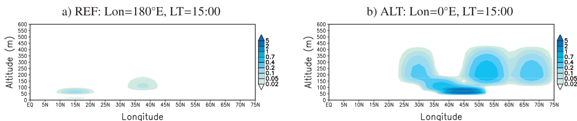
Fig. 14. Methane clouds as a function of latitude and altitude above the surface, around July 14, 2015, in a) the reference simulation ( N_2 only in Sputnik Planum) at longitude 180^\circ E and Local Time 15:00, and b) the alternative simulation (with surface N_2 ice between 35^\circ N and 48^\circ N ) at longitude 0^\circ E and Local Time 15:00.
