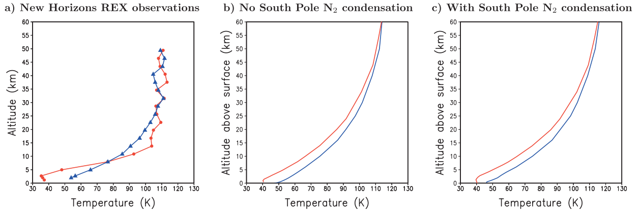
Fig. 6. Comparison of the two temperature profiles retrieved by the New Horizons REX experiment (Hinson et al., 2015b; Gladstone et al., 2016) at 193.5°E, 17.0°S and Local time 16:31 (red) and 15.7°E, 15.1°N and Local time 04:42 (blue) with GCM results. The model data are taken at the same location and time, except for the profile at latitude 17.0°S which is shifted to 7.5°N in order to locate it just within the modeled Sputnik Planum basin filled with N 2 ice, as it is the case in reality (see text). (For interpretation of the references to colour in this figure legend, the reader is referred to the web version of this article.)
