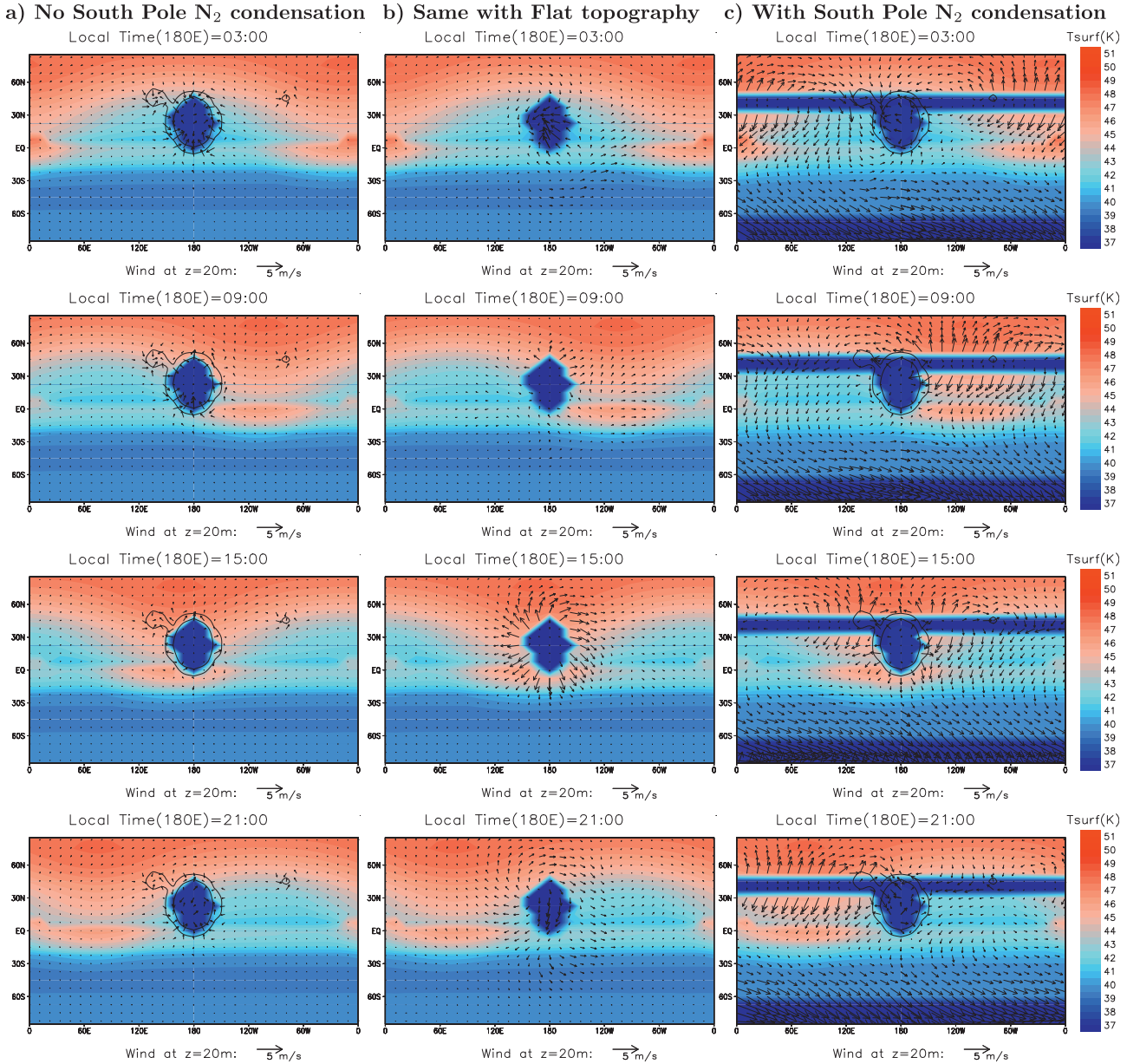
Fig. 3. Maps of surface temperature and winds at 20 m above the surface in July 2015 at different local times for 3 simulations: a) the reference simulations with no N_2 condensation at the south pole, b) The same simulation with flat topography (started from the reference run on January 1st, 2015, and analyzed on July 14, 2015) c) the alternative simulation with N_2 condensation at the south pole. From top to bottom, the local time LT in the middle of the map (longitude 180^\circ ) is 3:00, 9:00, 15:00 and 21:00, with LT (hours) = [longitude ( ^\circ ) - subsolar point longitude ( ^\circ )]/15 + 12.
