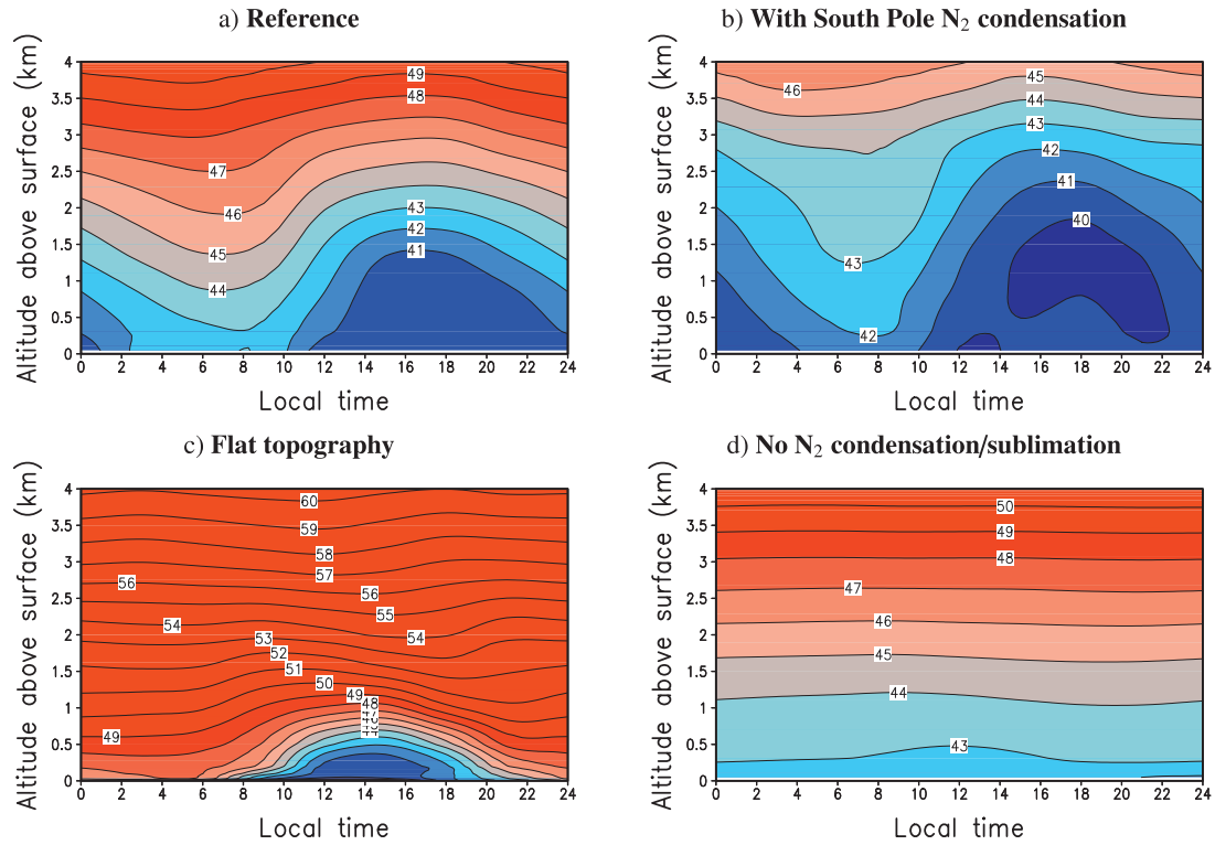
Fig. 7. Diurnal variations of atmospheric temperature in the lower atmosphere at 193.5°E–7.5°N (at the bottom of the modeled Sputnik Planum basin) for (a) the reference simulation (without South Pole N_2 condensation), (b) the alternative simulation (with South Pole N_2 condensation), (c) a version of the reference simulation with a flat topography, and (d) No N_2 condensation/sublimation at all on the planet. The simulations with flat topography and No N_2 condensation/sublimation were started from the reference run initial state on January 1st, 2015, and analyzed on July 14, 2015.
