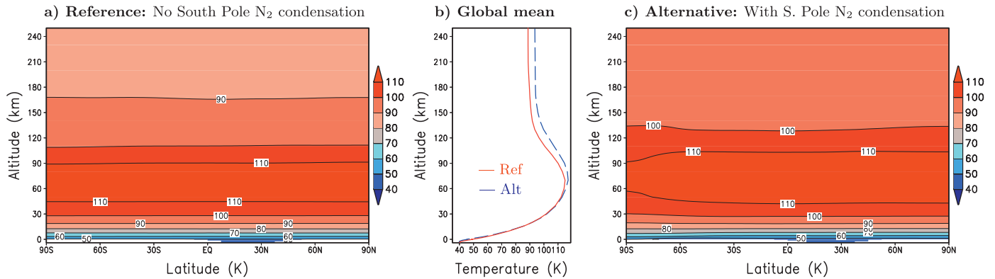
Fig. 5. Zonal-mean temperatures (K) in (a) the reference and (c) the alternative simulations in July 2015. The central plot (b) shows the global mean temperature profiles.
