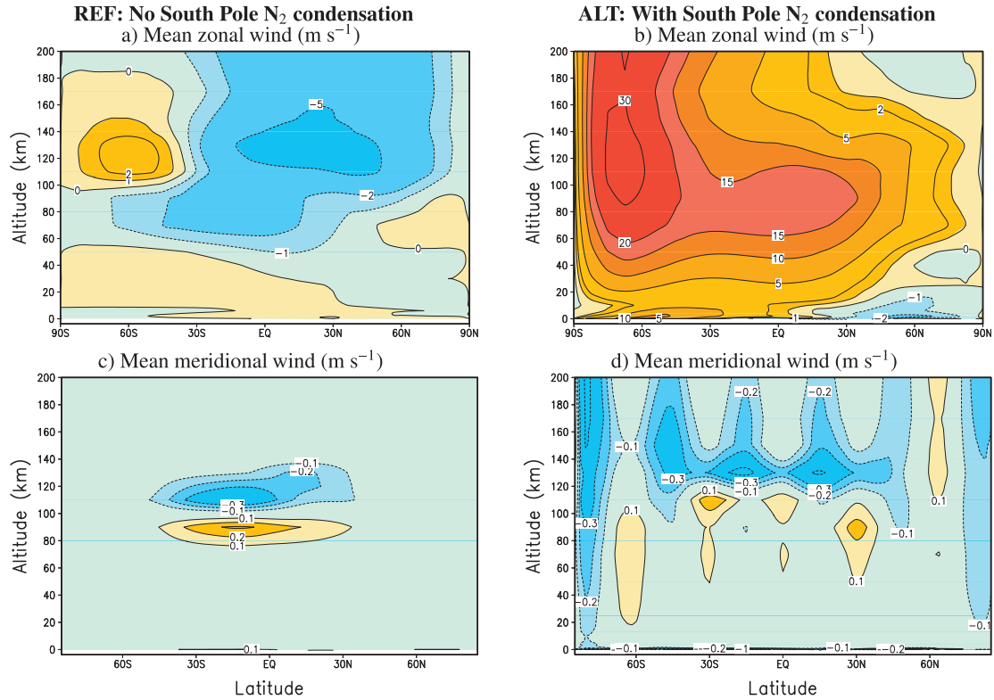
Fig. 10. Zonal-mean zonal and meridional winds ( \text{m s}^{-1} ) in the reference and alternative simulations in July 2015.
