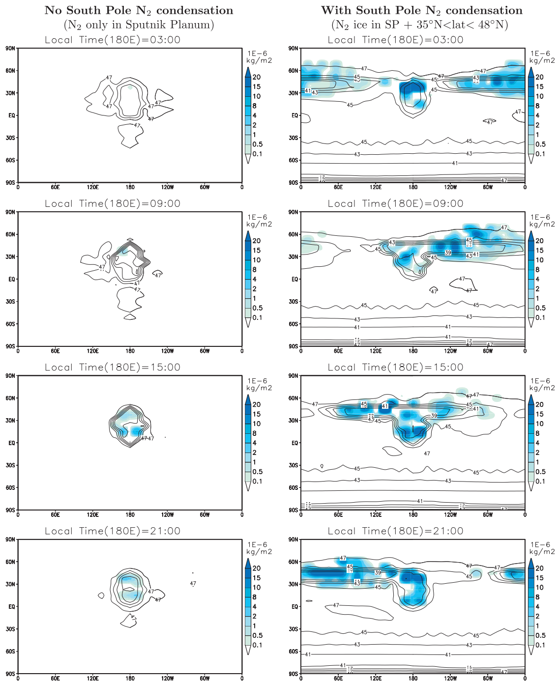
Fig. 13. Maps of methane ice clouds mass ( 10^{-6} kg per m^2 ) in July 2015 for the reference and alternative simulations for different local times at center of the map ( 180^\circ E ). The black contours show the atmospheric temperature 20 m above the surface.
