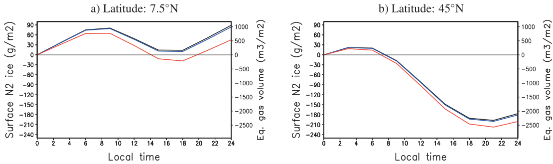
Fig. 8. Diurnal variation of the surface N_2 ice loading at two different latitudes in the modeled “Sputnik Planum” basin in July 2015. The right axis illustrates the corresponding volume of N_2 gas, assuming a pressure of 1 Pa and a temperature of 40 K. The different line colours correspond to different kinds of simulations: reference (blue), alternative with South Pole N_2 condensation (black, partly hidden by the blue line), and with a flat topography (red). The curves do not loop (i.e. the values at 24:00 differ from the values at 0:00) because every Pluto day the integrated surface budget corresponds to a net gain of N_2 ice by condensation at 7.5°N and a net loss by sublimation at 45°N, where the incident solar flux is stronger than at 7.5°N. (For interpretation of the references to colour in this figure legend, the reader is referred to the web version of this article.)
