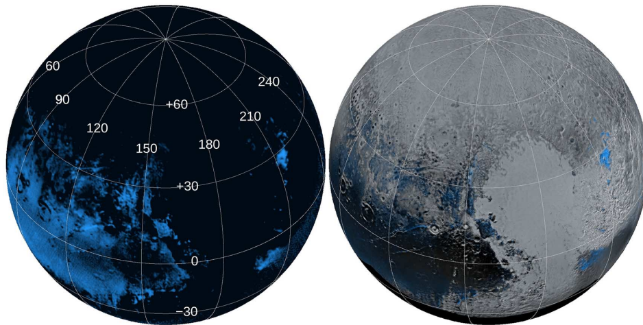
Fig. 2. LEISA map of Pluto's nonvolatile H 2 O ice. Left: Map showing the correlation coefficient between each LEISA spectrum and a template Charon-like H 2 O ice spectrum [e.g., (47,49)], highlighting where H 2 O absorption is least contaminated by other spectral features. Right: LEISA map superposed on the reprojected LORRI base map.
