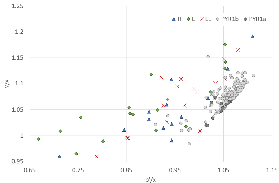
Figure 11. Scatterplot with ratio of v/x filters on the Y-axis and b'/x filter on the X-axis for PYR1a and PYR1b boulders. Resampled laboratory spectra of 57 OCs (H, L, and LL types) are also shown on this plot with different symbols. The color properties of some boulders are similar to those of OCs suggesting a compositional affinity.
