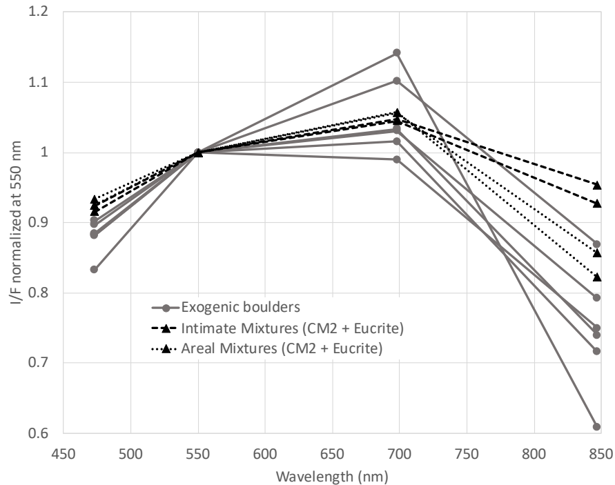
Figure 7. MapCam color spectra of exogenic boulders belonging to the PYR1b class with W_{\text{peak}} > 10\% , and a selection of resampled laboratory spectra of eucrite (Millbillillie) and CM2 carbonaceous chondrite (Murchison) intimate (30 and 40% CM2) and areal (70 and 80% CM2) mixtures. I/F was normalized at 550 nm. Color spectra of the mixtures match some of the exogenic boulders, suggesting that some might have a dusting of carbonaceous material from Bennu.
