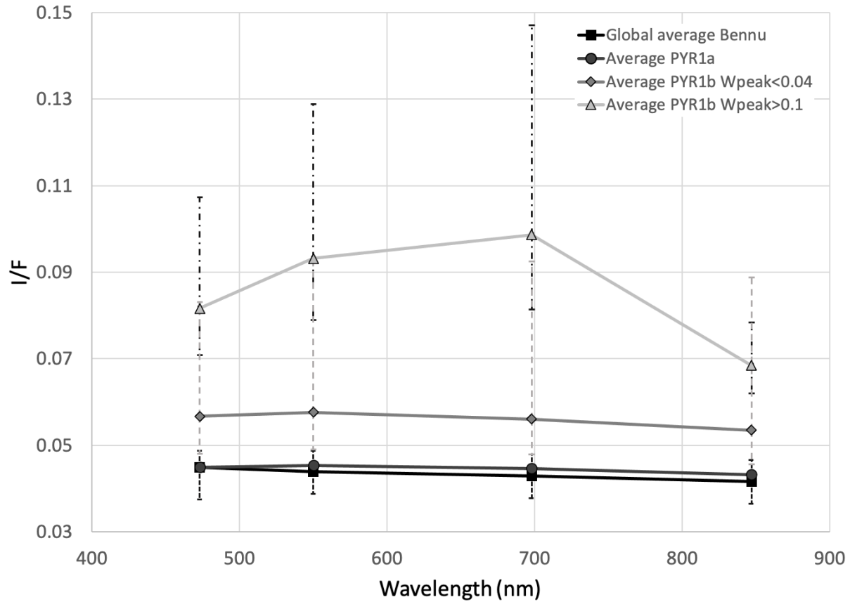
Figure 3. (A) Average MapCam spectra of PYR1a and PYR1b (high and low W_{\text{peak}} sub-groups separated) with the pyroxene-like absorption feature along with the global average spectrum of Bennu. Error bars indicate the highest and lowest values found in each filter for each group of boulders: dash-dot line for PYR1b with W_{\text{peak}} > 10\% , grey dashed line for PYR1b with W_{\text{peak}} < 4\% , and black dashed line for PYR1a. (B) Same data but normalized at 550 nm. (C) Average MapCam spectra of PYR2a and PYR2b normalized at 550 nm compared with the global average spectrum of Bennu.
