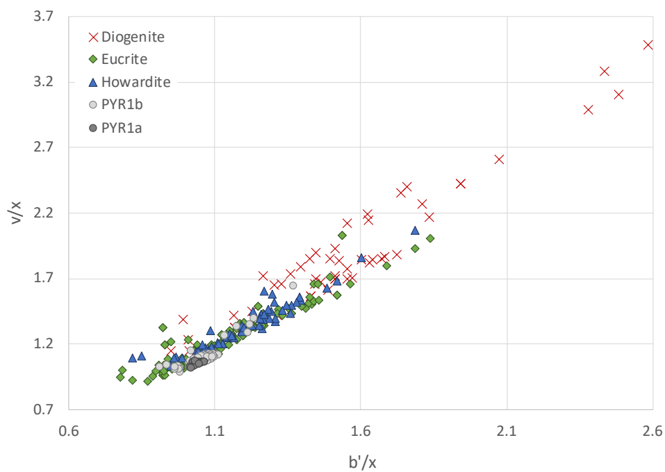
Figure 6. Scatterplot with the ratio of v/x filters on the Y-axis and b'/x filter on the X-axis for PYR1a and PYR1b boulders. Resampled laboratory spectra of 255 HED meteorites from asteroid (4) Vesta are also shown using different symbols. Color ratios of PYR1a and PYR1b boulders are similar to those of eucrite meteorites, suggesting a compositional affinity.
