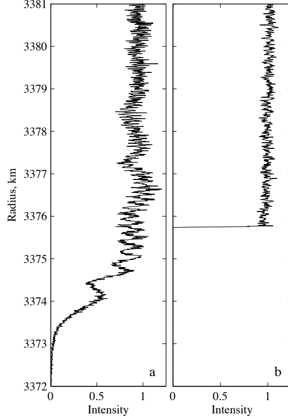
Figure 3. Measurements of signal intensity during a radio occultation experiment conducted with Mars Global Surveyor on 31 December 1998. (a) Original data with a sample spacing of approximately 5 m. The diffraction pattern produced by the surface of Mars contains > 40 diffraction fringes and extends more than 5 km beyond the limb of Mars. Refractive bending in the lower atmosphere deflects the diffraction pattern into the geometric shadow of Mars by \approx 2 km. (b) Intensity measurements after inverse Fresnel filtering. Abrupt drop in intensity marks the location of the surface.
