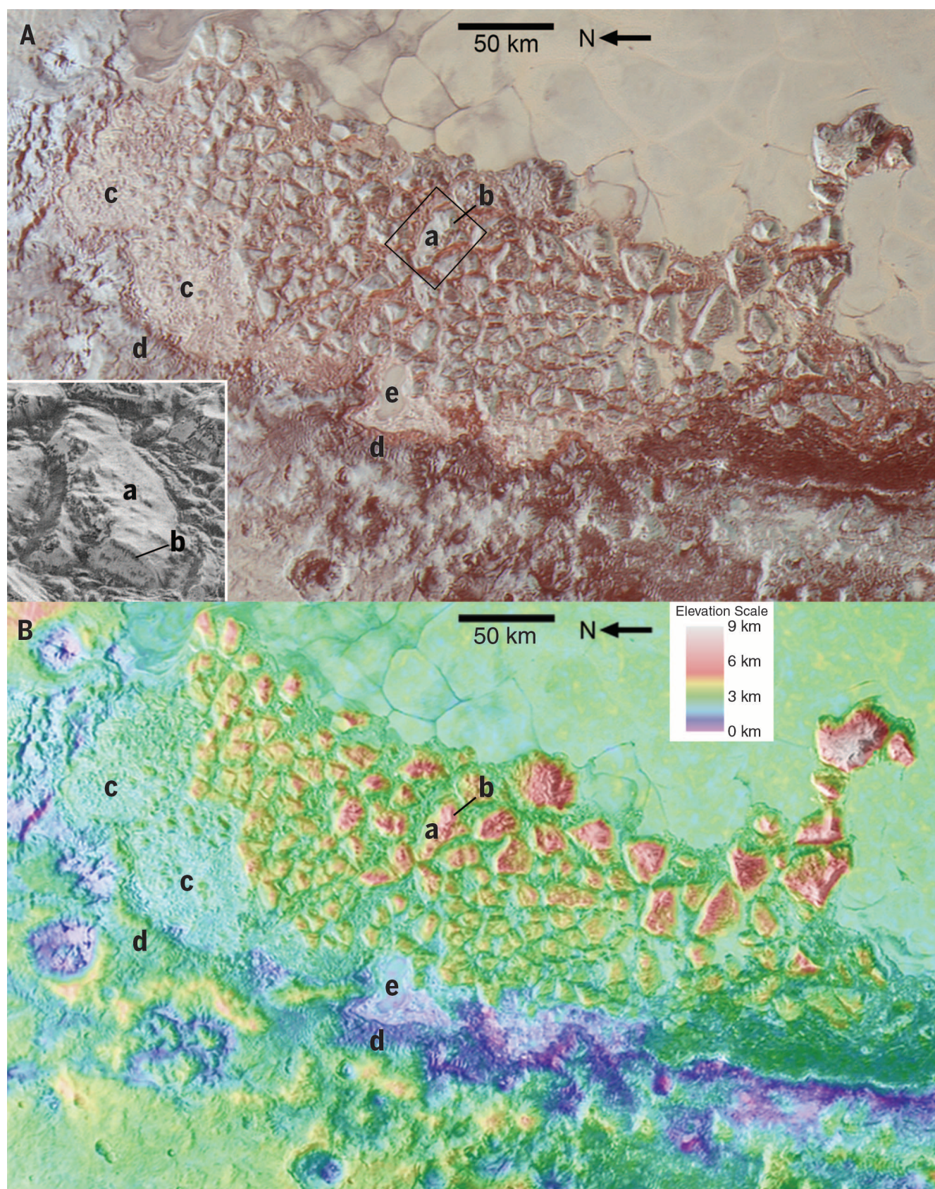
Fig. 2. The chaotic mountains of al-Ildrisi Montes on the northwest margin of SP. (A) Image is 680 m/pixel, reprojected, MVIC enhanced color coverage of the P_COLOR2 observation, centered at 34.5°N, 155°E. The 30 by 40 km-wide inset shows a detail of one mountain in 79 m/pixel, LORRI coverage of the P_MVIC_LORRI_CA observation. (B) Colorized digital elevation model (DEM) overlain on the 680 m/pixel MVIC coverage. (a) Textured surface possibly predating block formation; (b) steep fracture surface with possible exposed layering; (c) chaos composed of small blocks; (d) inward-facing terraces; (e) small exposure of SP-like material.
