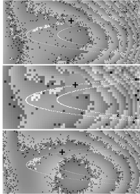
Fig. 8. Possible clumps seen in the ring. This series of three images was taken near \alpha = 1^\circ , with a 90-sec delay between the first image pair and a 160-sec delay between the second pair. All images are in the clear filter; the central image was taken in the SUM2 mode causing its larger pixel size. Resolution is 115 \text{ km pix}^{-1} except for the middle frame, which is 230 \text{ km pix}^{-1} . The ring boundaries are marked, as is the position of Adrastea (masked out, behind the +). Keplerian motion over this interval would move the clumps \sim 4^\circ in longitude; the ring images span \sim 40^\circ of longitude. The material appears to move in the forward keplerian direction; however, it is difficult to ascertain the clumps’ true nature from these images alone.
