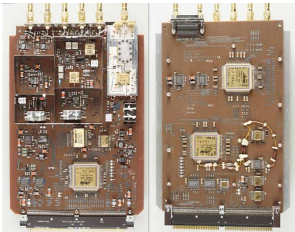
Figure 3- Photographs of Uplink Card
