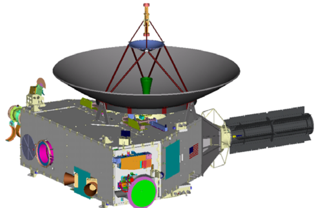
Figure 1 The New Horizons Spacecraft
