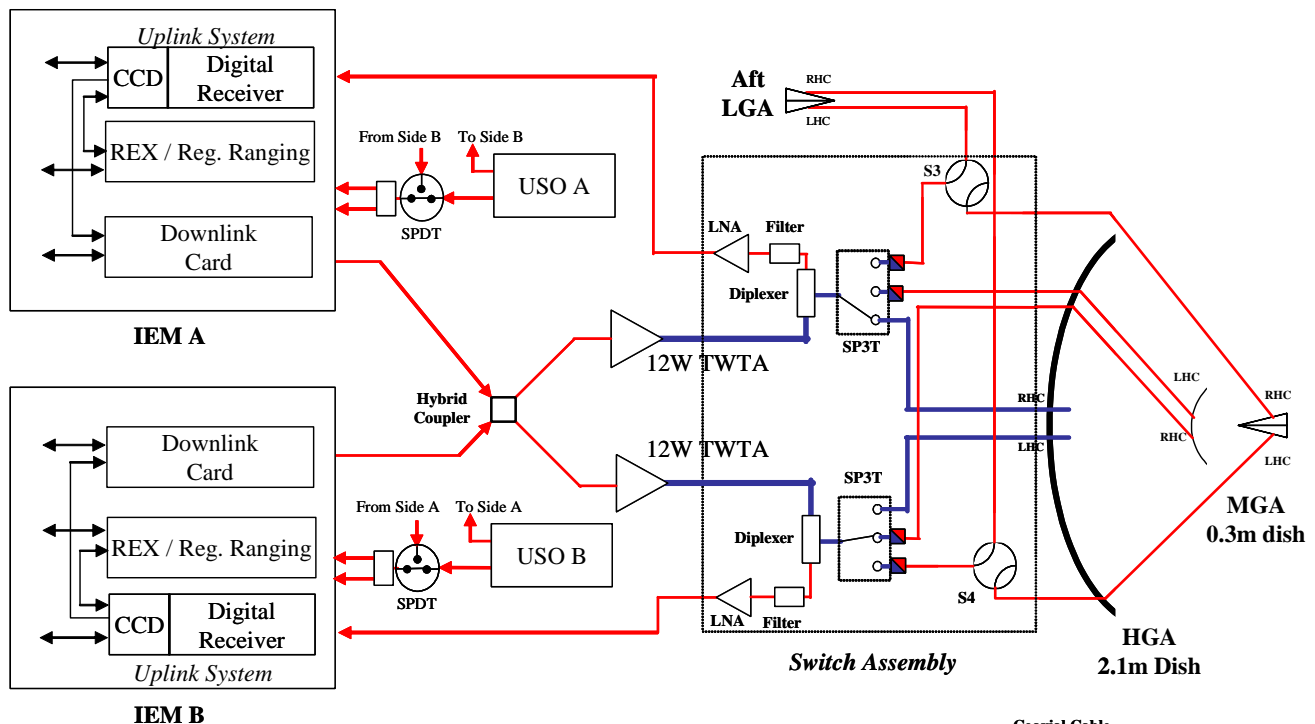
Figure 2 Telecommunications System Block Diagram
