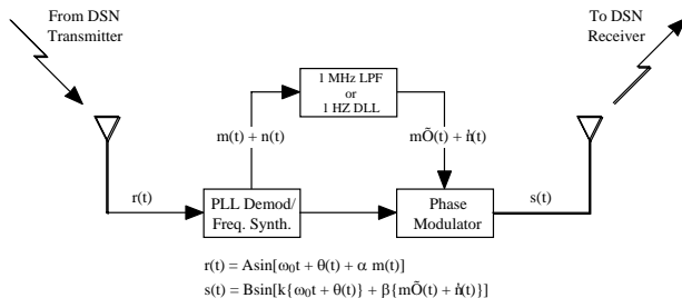
Figure 7 Signal Processing for Spacecraft Tracking
