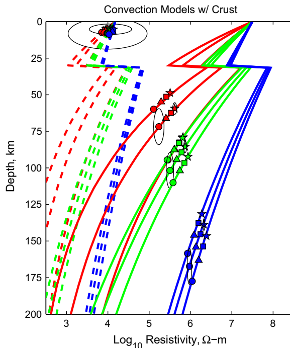
Fig. 9. Point soundings for convection models with conductive crust superimposed. Compare to Fig. 6.
