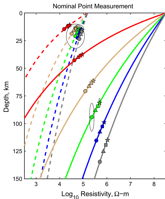
Fig. 5. Dry (solid) and “wet” (dashed) electrical resistivity vs. depth for specified lithospheric thicknesses of L = 100 – 500 km at 100-km increments (red through gray, respectively). Symbols show resistivity structure inverted at the first four Schumann resonances ( \sim 10 to \sim 32 Hz; lowest frequency penetrates deepest). Error ellipses at representative L = 300 km and 1st and 4th resonances indicate effect of nominal instrumental errors on resistivity-depth recovery. Random errors are larger for wet resistivity due to smaller induced fields. These calculations represent point measurements without horizontal averaging. (For interpretation of the references to color in this figure legend, the reader is referred to the web version of this article.)
